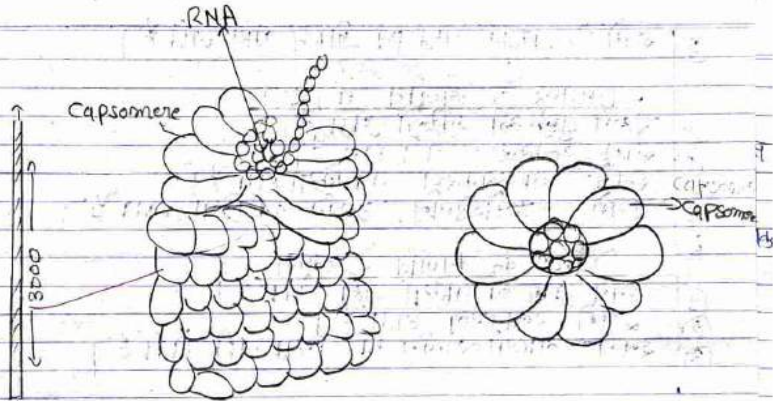
Ultrastructure of TMV
